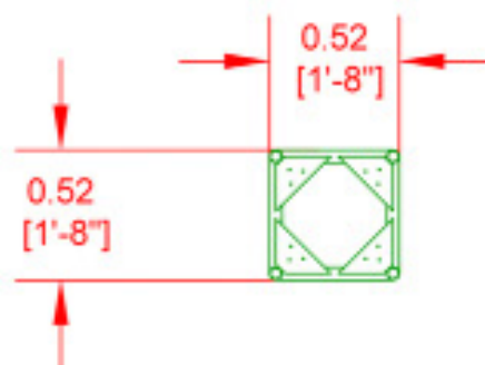
Corner Block
