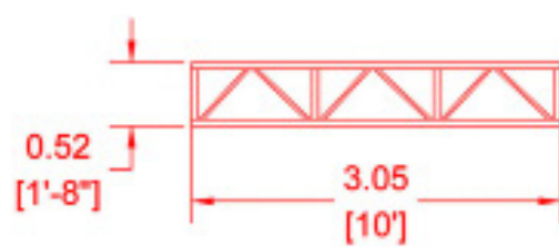
Truss 10 FT
