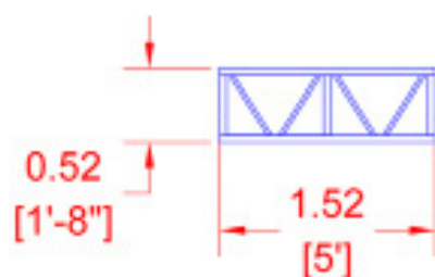
Truss 5 FT
