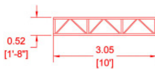
Truss 10 FT
