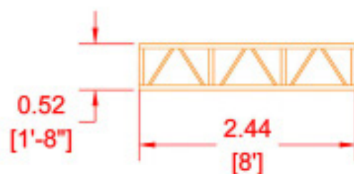
Truss 8 FT
